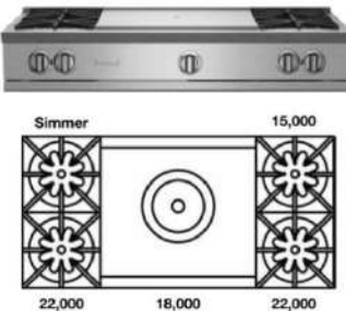
48" Nova (RNB) Rangetop with 24" French Top
