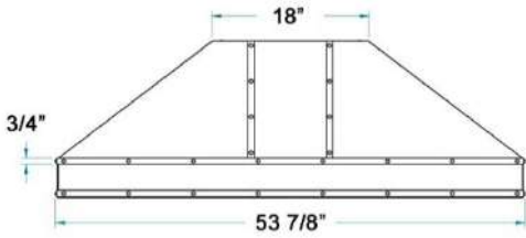
54" Dimensions
