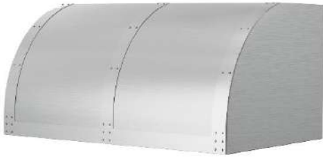
30" & 36" Bonanza Wall Hood Standard Height: 18" | Standard Depth: 24"
