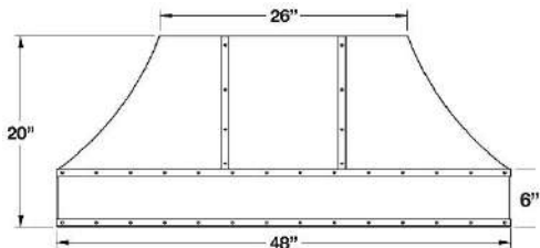
48" Dimensions
