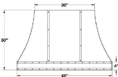
48" Dimensions
