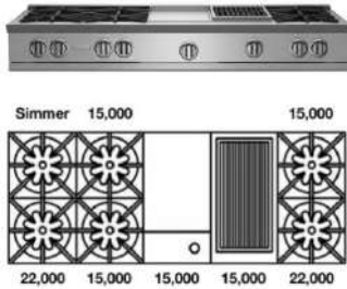
60" Nova (RNB) Rangetop with 12" Griddle & Charbroiler
