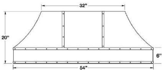
54" Dimensions
