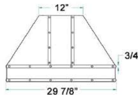
30" Dimensions
