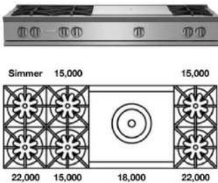
60" Nova (RNB) Rangetop with 24" French Top
