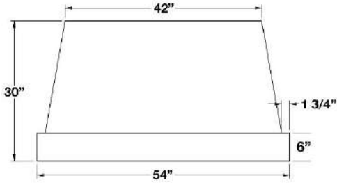
54" Dimensions
