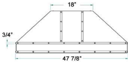
48" Dimensions
