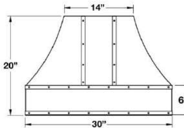
30" Dimensions
