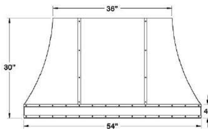
54" Dimensions
