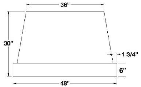
48" Dimensions
