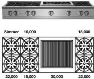
60" Nova (RNB) Rangetop with 24" Charbroiler
