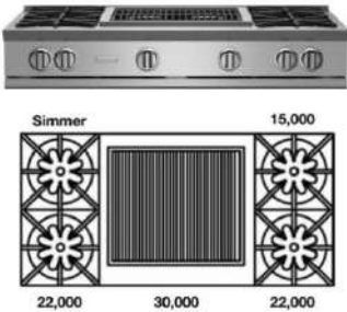
48" Nova (RNB) Rangetop with 24" Charbroiler
