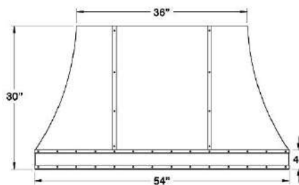
54" Dimensions
