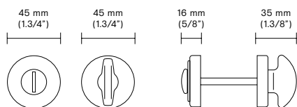
RP Round rosette 45 mm (1.3/4") Thumb turn (Interior and emergency release)
