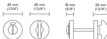
Interior and emergency release with indicator
