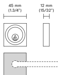
RQ Square rosette with cylinder collar
