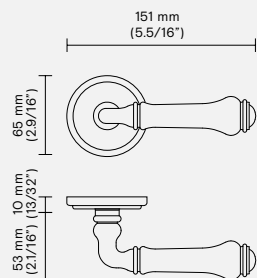
Standard option (mm/inches) RT Traditional rosette
