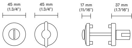
RPS Round rosette Stainless steel 45 mm (1.3/4") Thumb turn (Interior and emergency release)
