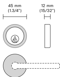
RP Round rosette with cylinder collar
