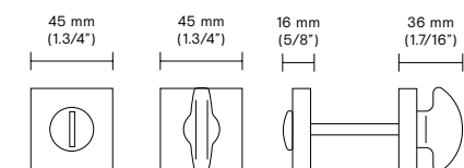
RQ Square rosette 45 mm (1.3/4") Thumb turn (Interior and emergency release)
