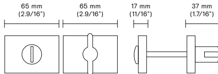
RQS Square rosette Stainless steel mm 65 (2.9/16") Thumb turn (Interior and emergency release)
