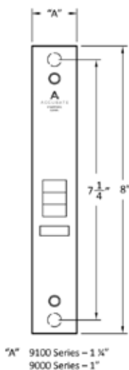
Lock front (shown ML-F function)
