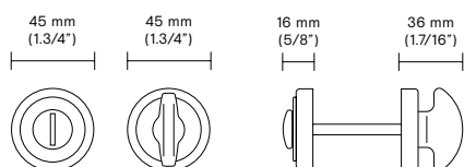
RT Traditional rosette 45 mm (1.3/4") Thumb turn (Interior and emergency release)
