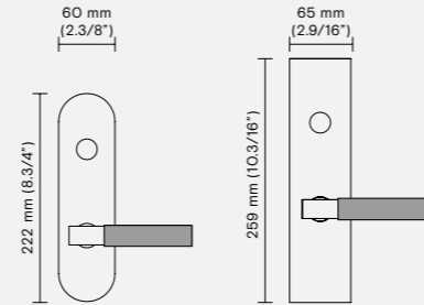
Escutcheon options (mm/inches) NES Oval plate ERS Rectangular plate
