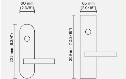
Escutcheon options (mm/inches) NES Oval plate ERS Rectangular plate
