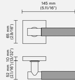
Standard option (mm/inches) RQS Square rosette
