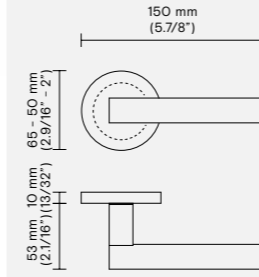
Standard option (mm/inches) RPS Round rosette - RSS Small 2" rosette
