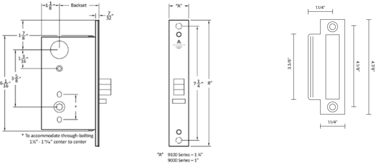
Lock body (shown ML-F function)
