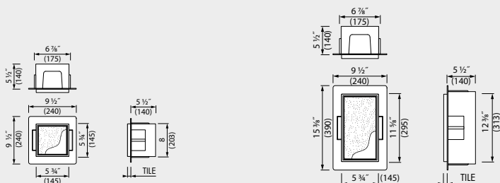
BOXT-T-15x15-14 | Wall niche / paper holder 6" x 6" (15 x 15 cm)
