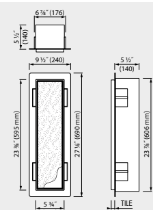
TCL-11 | Built-in waste container & wall niche
