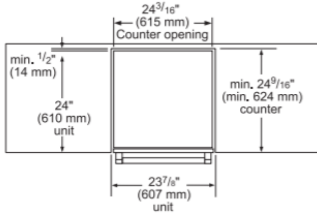
Thermador double drawer under counter top dimension. (Unit door flushed with the cutout)
