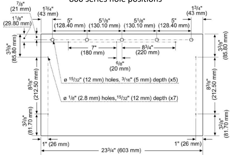
800 series hole positions
