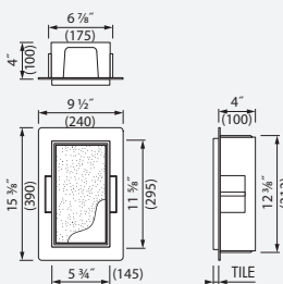
Depth 4" (100 mm)
