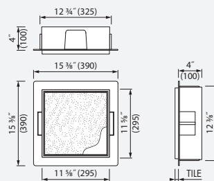
Depth 4" (100 mm)
