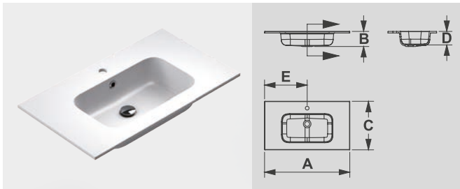
MINERAL SOLID® Ref. 168873 $ 795.00 A: 805 mm B: 143 mm C: 460 mm D: 128 mm E: 400 mm
