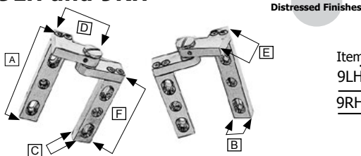
Solid Brass Removable Pin Intermediate Pivot Hinge
