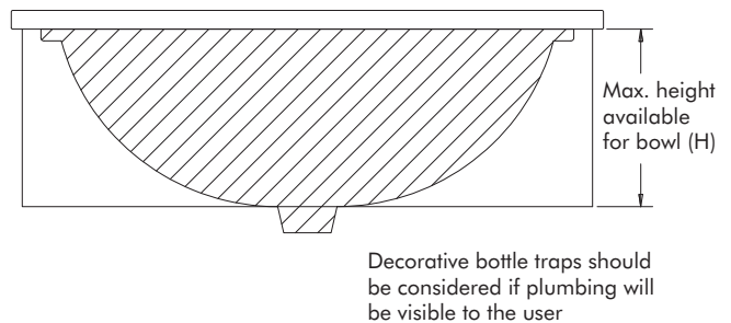
Front View of 7-1/2" (H1) Tip Out Vanity
