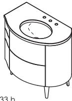
36 x 22 x 33 h MB135SX vanity MB135TSX countertop 33S lavatory
